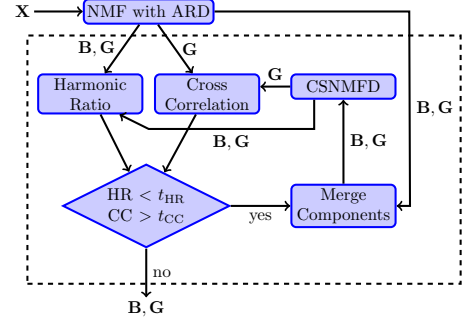
Fig. 4. Signal flow of the proposed algorithm.
