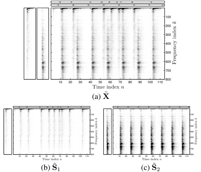
Fig. 1. Example of successful source separation with NMFD for a mixture of sources with temporal structure.
