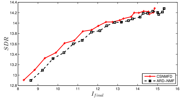
Fig. 7. NMF with ARD compared to the proposed algorithm. I_{final} is the average resulting number of components.
