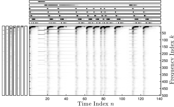
Fig. 5. Result of NMF with ARD for a mixture of saxophone and bass drum.
