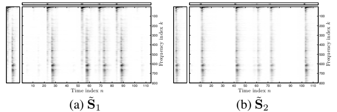
Fig. 2. Example of unsuccessful source separation with NMFD for a mixture of sources with temporal structure.
