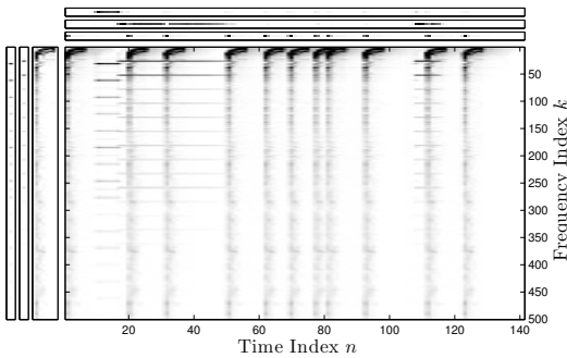
Fig. 6. Result of the algorithm using CSNMFD for a mixture of saxophone and bass drum.
